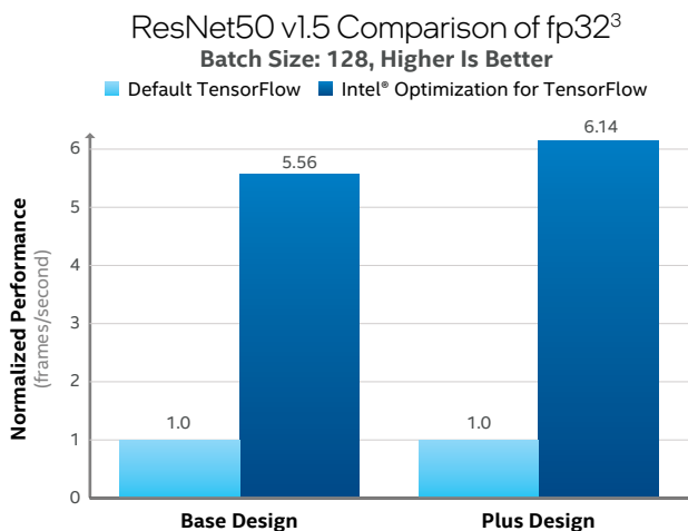
Figure 3. The Intel® Optimization for TensorFlow provides up to a 6.14x throughput improvement compared to the default TensorFlow framework.
